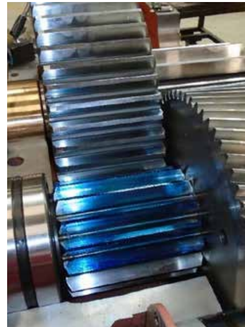
Gearbox refurbishment
